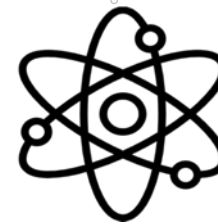
Quantum Sensing
